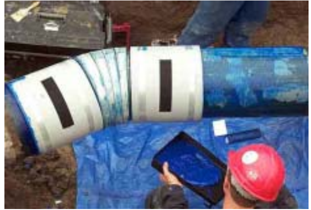
In the photo above, a sleeve is applied to both ends of the bend repair area, butted next to the girth weld. The void in the girth weld area will be filled using WrapMaster's PermaPutty high compressive filler material. Two PermaWrap sleeve will be applied over the girth weld areas to be reinforced.
